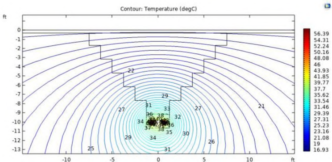
Figure 1 – Temperature profile
