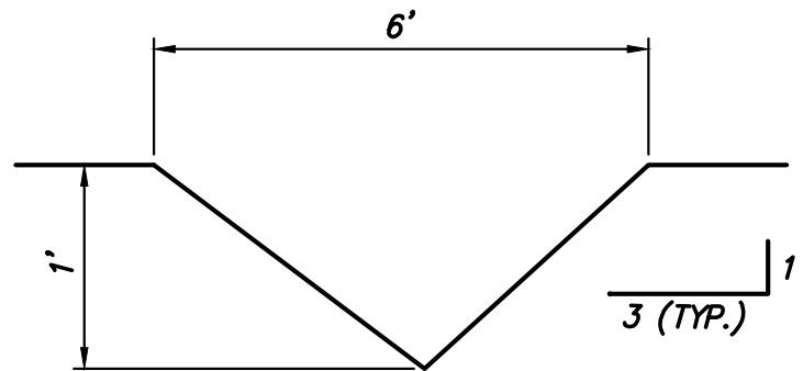
TEMP. SWALE CROSS SECTION 405-1, 405-2, AND 405-3 NOT TO SCALE
