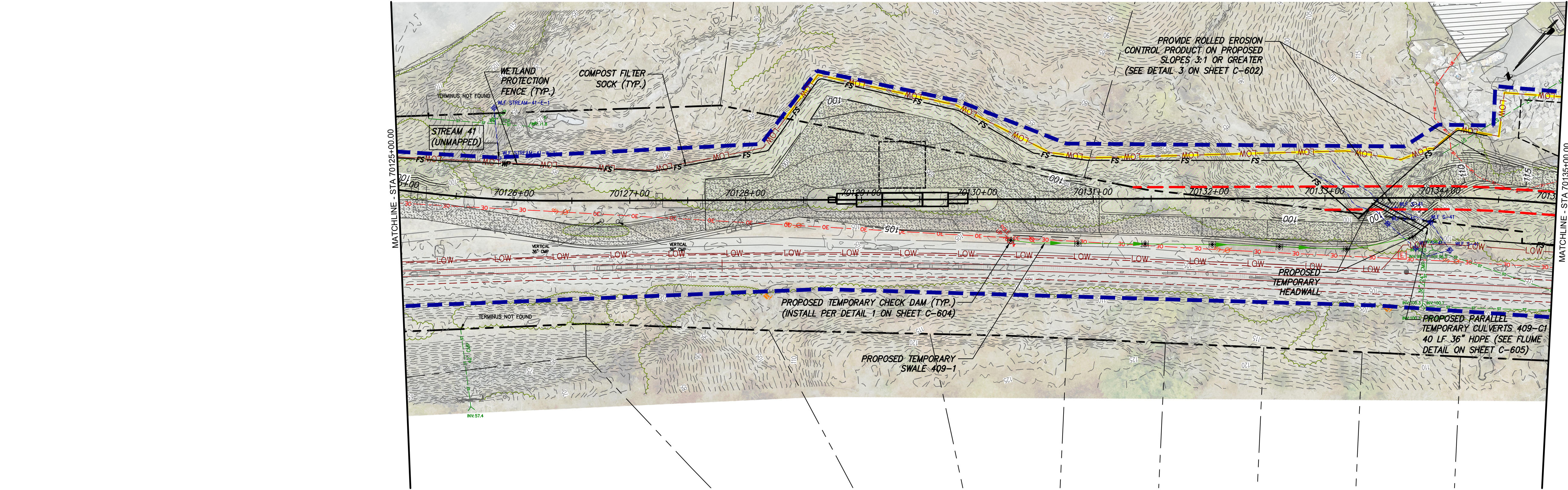
STA. 70125+00.00 TO 70135+00.00 PLAN VIEW SCALE: 1" = 50'
