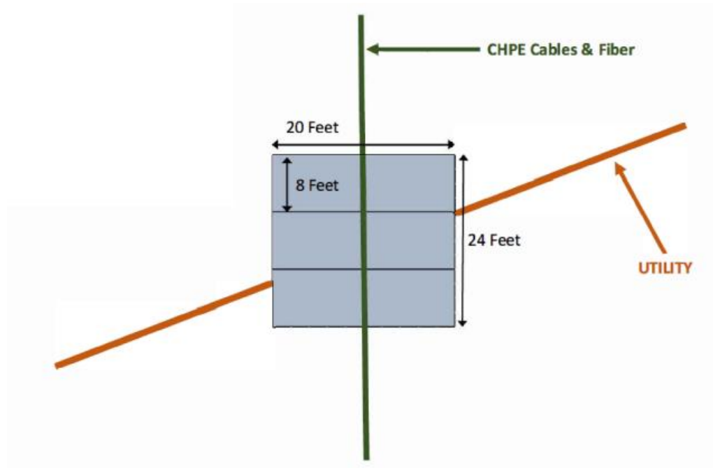
Figure 2 Indicative arrangement of pre-lay mattresses over existing utility
