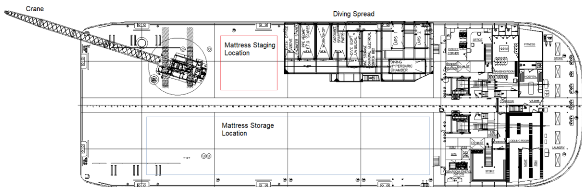
Figure 12 Indicative Diver Assisted Mattress Installation Spread
