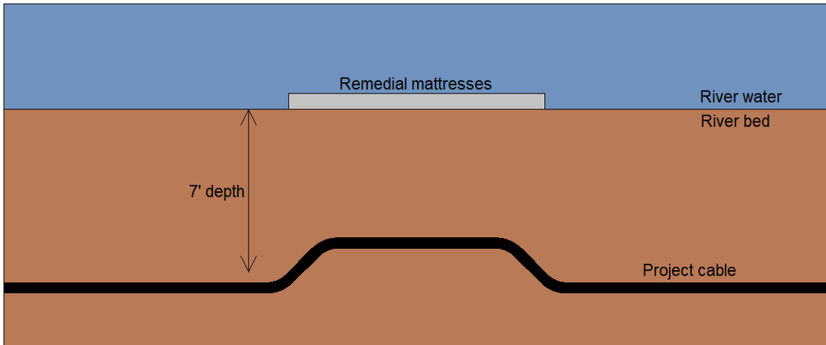
Figure 4 Indicative remedial mattressing drawing
