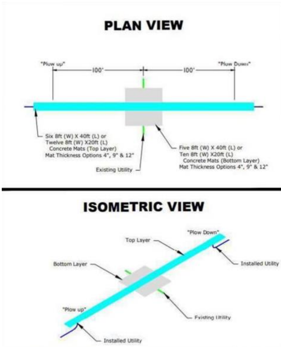
Figure 3 Indicative arrangement of post-lay mattressing over project cable
