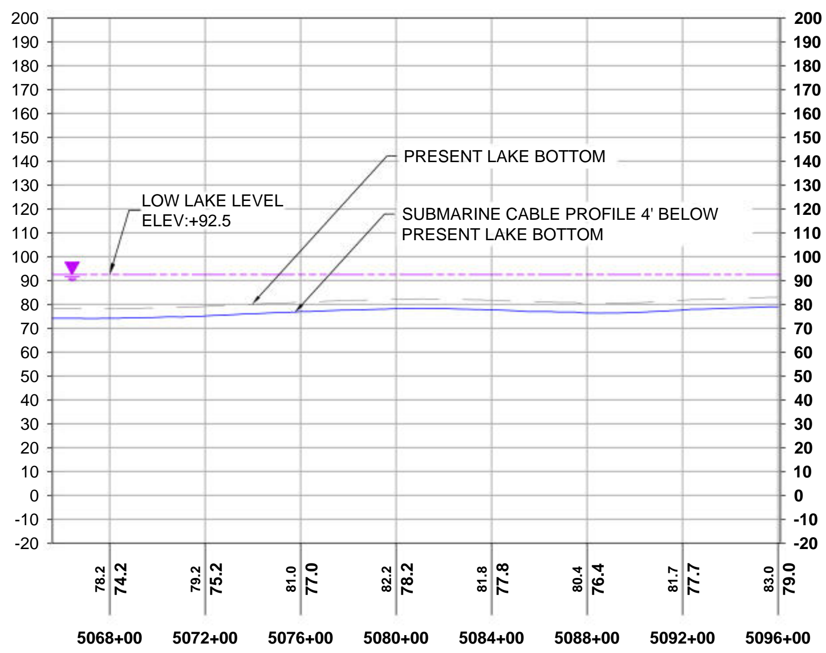
2 PROFILE VIEW HORIZONTAL SCALE: 1"=400', VERTICAL SCALE: 1"=40'
