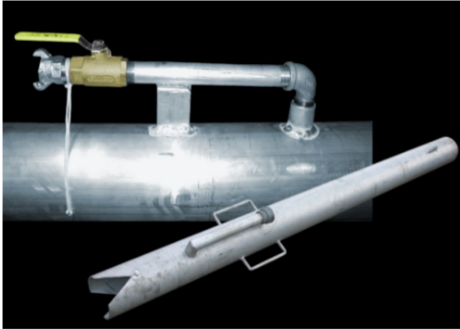
Figure 22 – Air-lift device (diver operated)
