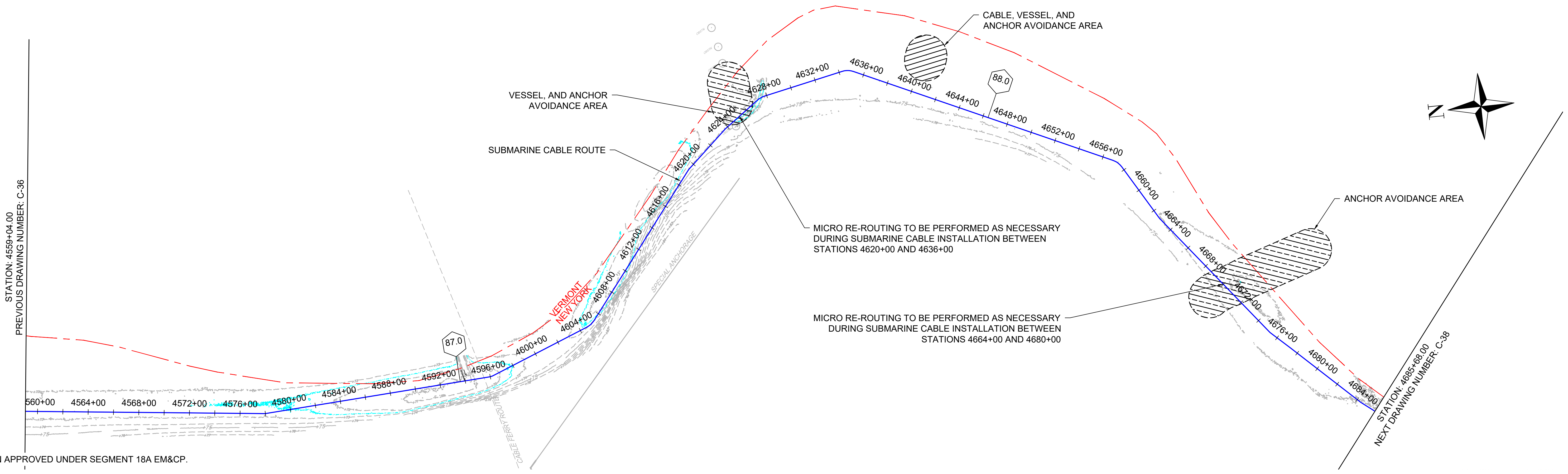
1 PLAN VIEW SCALE: 1"=400'
