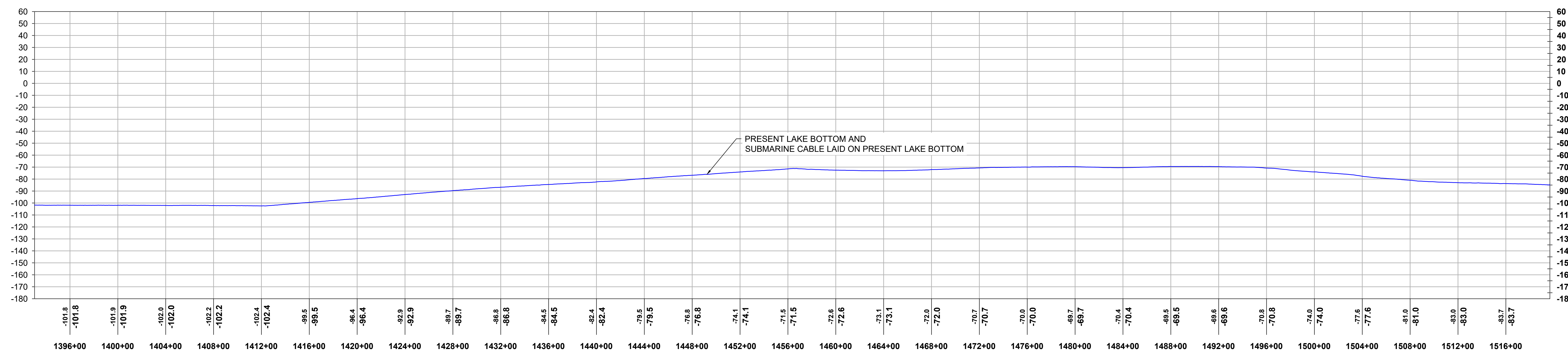
2 PROFILE VIEW 18 HORIZONTAL SCALE: 1"=400', VERTICAL SCALE: 1"=40'
