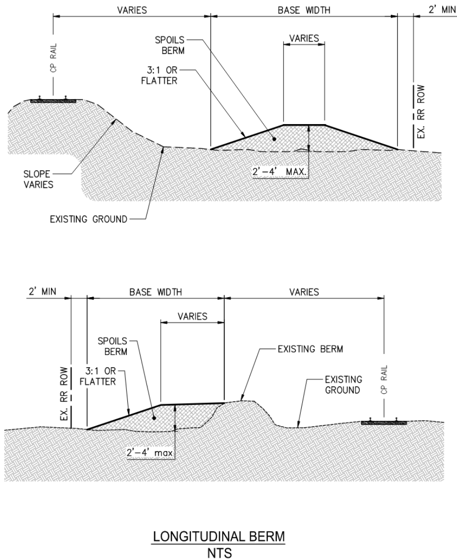
Figure 7.4 – Longitudinal Berm
