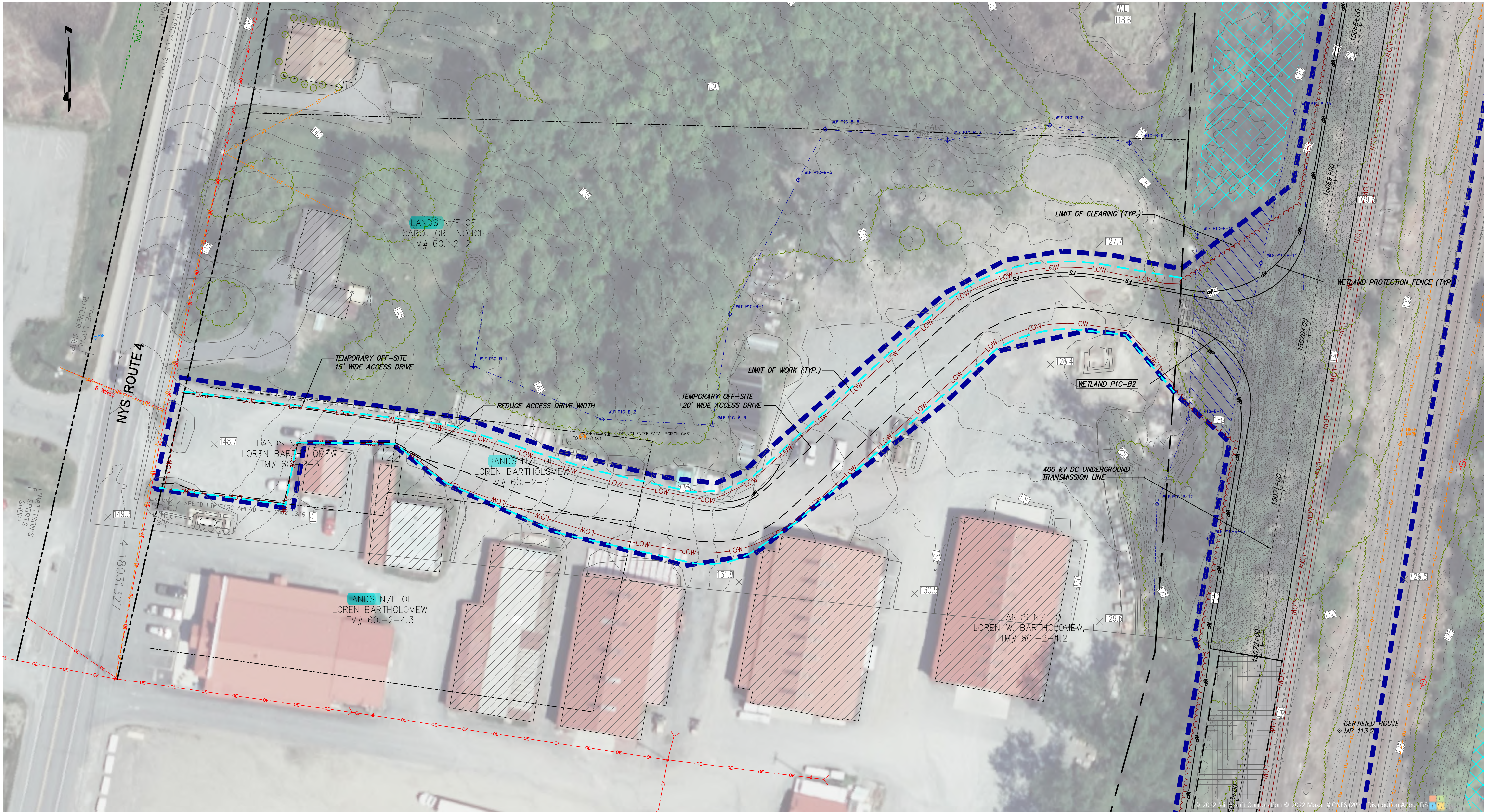
ACCESS ROAD OFF NYS ROUTE 4 AT STA 15069+00± SCALE: 1" = 30'
