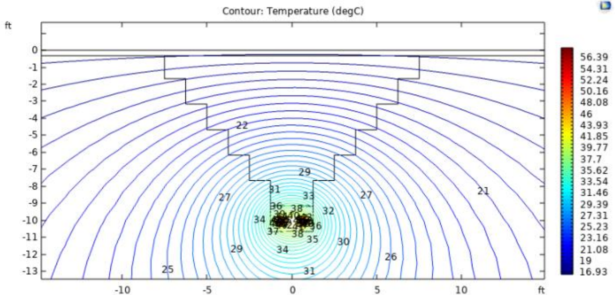
Figure 1 – Temperature profile
